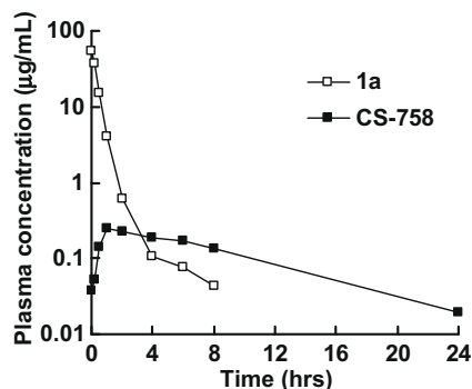
Figure 4. Plasma level of CS-758 after iv administration of 1a to rats at a dose of 2 mg/kg (average of three rats).
