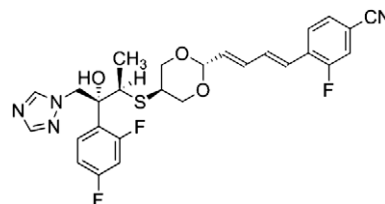
Figure 1. Structural formula of CS-758.
