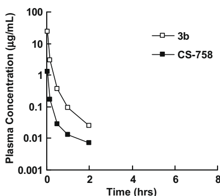
Figure 5. Plasma level of CS-758 after iv administration of 3b to rats at a dose of 2 mg/kg (average of three rats).
