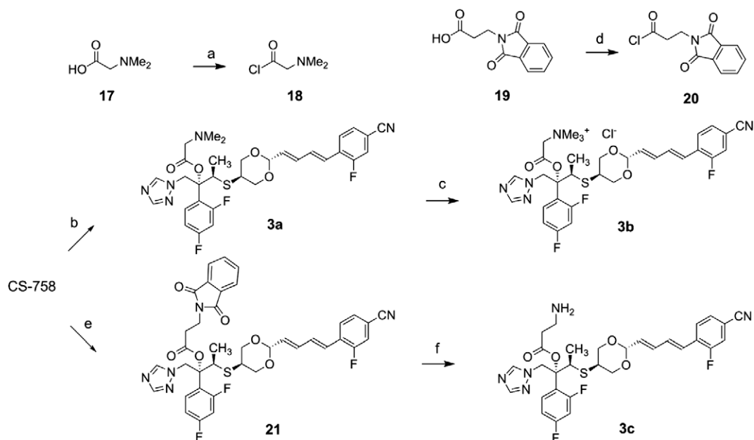
Scheme 5. Synthesis of compound 1c 's derivatives 3a–c . (a) (\text{COCl})_2 , cat. DMF, THF; (b) NaH, 18 , THF, 37%; (c) 1-MeOTf, i -Pr 2 NEt, CH 2 Cl 2 , 2-DOWEX1 × 4 (Cl form), 32%; (d) (\text{COCl})_2 , cat. DMF, CH 2 Cl 2 ; (e) NaH, 20 , THF, 10%; (f) MeNHNH 2 , CH 2 Cl 2 , 61%.
