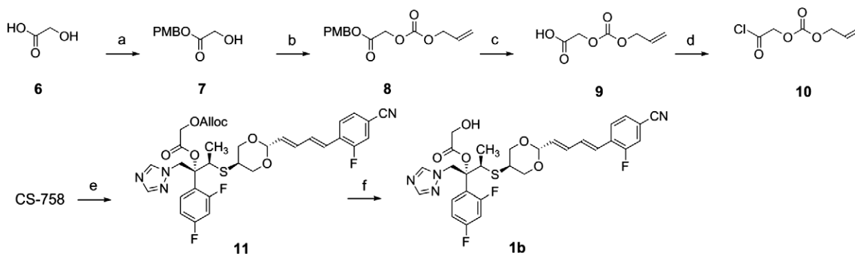
Scheme 2. Synthesis of 1b . Reagents and conditions: (a) 1- \text{NaHCO}_3 , \text{H}_2\text{O} , 2-(4-( \text{MeO} ) \text{BnCl} ), 60%; (b) allyl chloroformate, DMAP, \text{CH}_2\text{Cl}_2 , 86%; (c) anisole, TFA, quant.; (d) (\text{COCl})_2 , cat. DMF, THF, 90%; (e) 1- \text{NaH} , THF; (f) 2-10 , 16%; (g) \text{PdCl}_2(\text{PPh}_3)_2 , n\text{-Bu}_3\text{SnH} , \text{CH}_2\text{Cl}_2 , quant.
