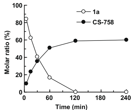
Figure 2. Conversion of 1a (○) to CS-758 (●) in human liver microsome.
