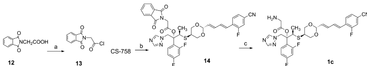
Scheme 3. Synthesis of 1c . Reagents and conditions: (a) (\text{COCl})_2 , cat. DMF, \text{CH}_2\text{Cl}_2 ; (b) \text{NaH} , 13 , 26%; (c) \text{CH}_3\text{NHNH}_2 , \text{CH}_2\text{Cl}_2 , 85%.
