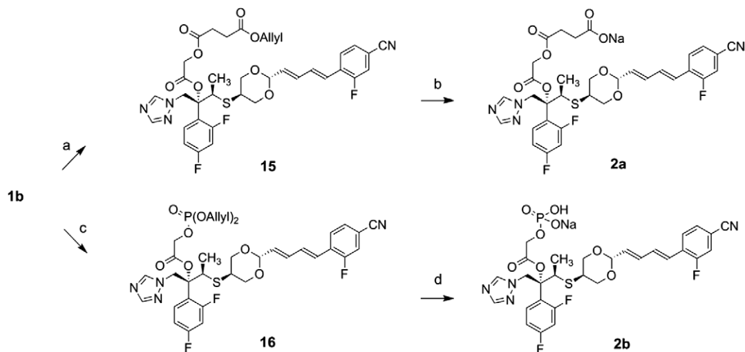
Scheme 4. Synthesis of compound 1b 's derivatives 2a and 2b . Reagents and conditions: (a) monoallyl succinic acid chloride, \text{NEt}_3 , DMAP, \text{CH}_2\text{Cl}_2 , 77%; (b) 1- \text{PdCl}_2(\text{PPh}_3)_2 , n\text{-Bu}_3\text{SnH} , \text{CH}_2\text{Cl}_2 , 2- \text{NaHCO}_3 aq, then C-18 reverse phase column, 34%; (c) 1- i\text{-Pr}_2\text{NP}(\text{OAllyl})_2 , 1 H -tetrazole, \text{CH}_2\text{Cl}_2 ; 2- t\text{-BuOOH} , \text{CH}_2\text{Cl}_2 , 84%; (d) \text{PdCl}_2(\text{PPh}_3)_2 , n\text{-Bu}_3\text{SnH} , \text{CH}_2\text{Cl}_2 then \text{NaHCO}_3 aq, 52%, two steps.
