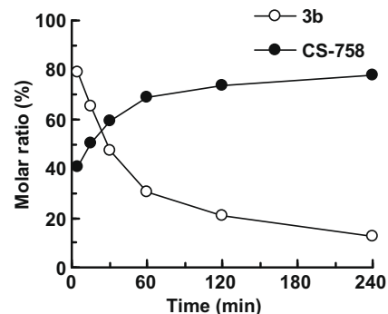
Figure 3. Conversion of 3b (○) to CS-758 (●) in human plasma.
