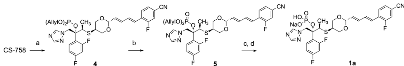
Scheme 1. Synthesis of 1a . Reagents and conditions: (a) i\text{-Pr}_2\text{NP}(\text{OAllyl})_2 , 1 H -tetrazole, \text{CH}_2\text{Cl}_2 , 89%; (b) t\text{-BuOOH} , \text{CH}_2\text{Cl}_2 , 82%; (c) \text{PdCl}_2(\text{PPh}_3)_2 , n\text{-Bu}_3\text{SnH} , \text{CH}_2\text{Cl}_2 ; (d) \text{NaHCO}_3 aq, then C-18 reverse-phase column chromatography, 45%, two steps.
